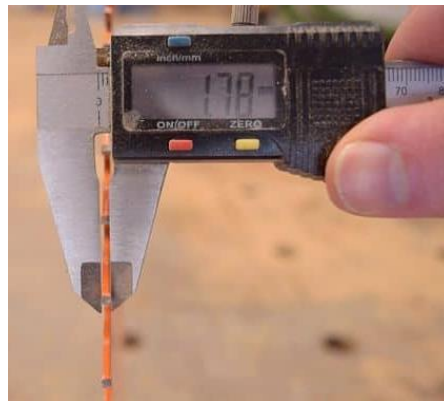
Figure 24: – Saw blade thickness measured by caliper
